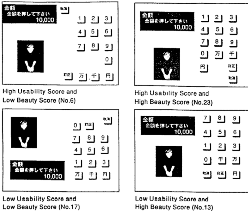
Figure 7-1. Sample layout patterns (source: Kurosu and Kashimura, 1995)
